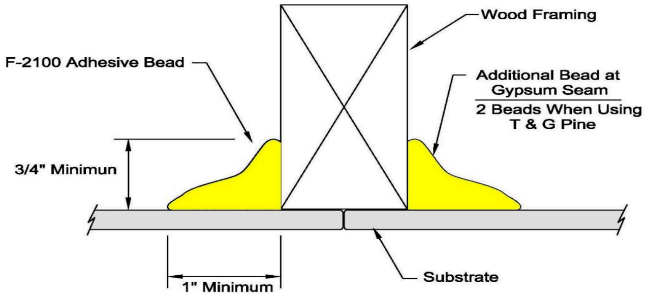
FIGURE 1—APPLICATION OF MIRACLE FOAMSEAL F-2100
